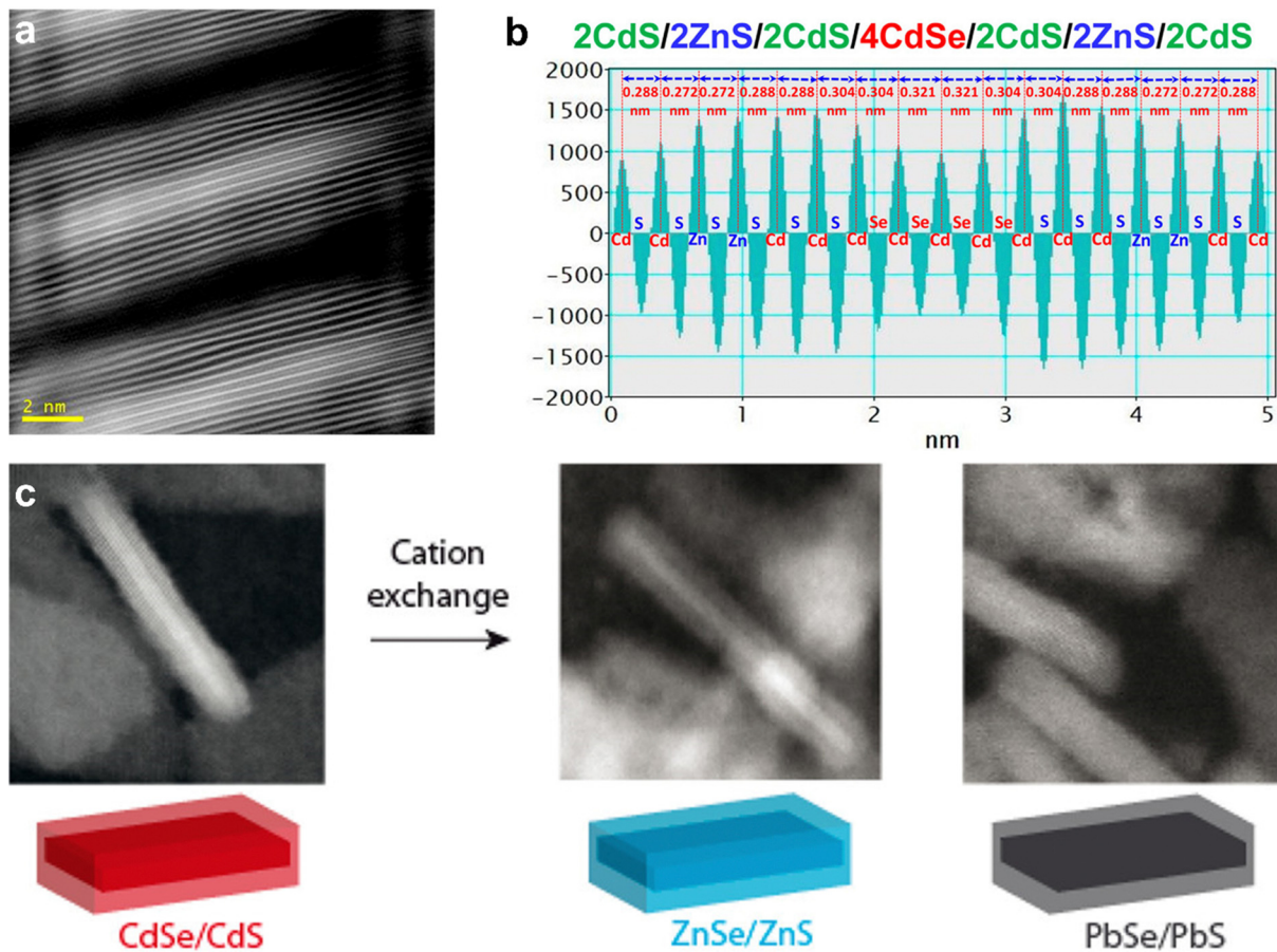
Fig. 11 (a) HAADF-STEM image of 2CdS/2ZnS/2CdS/4CdSe/2CdS/2ZnS/2CdS formed by c -ALD using Li 2 S/Li 2 Se and anhydrous Cd(HCOO) 2 /Zn(OAc) 2 powders as the sources of chalcogen and metal precursors, respectively; (b) the interplanar distances for this structure shown in (a); (c) schematic representation of the cation exchange of CdSe/CdS core/shell NPLs to ZnSe/ZnS and PbSe/PbS NPLs with corresponding HAADF-STEM images. Panels (a) and (b) are adapted with permission from The American Chemical Society. 240 Panel (c) is adapted with permission from The American Chemical Society. 254
