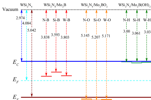
Fig. 7 Work function alignment of WSi_2N_4 , WSi_2N_4/Mo_2B , WSi_2N_4/Mo_2BO_2 and WSi_2N_4/Mo_2B(OH)_2 . The blue, cyan and wine solid lines represent the CBM, Fermi level and VBM of pure WSi_2N_4 . The red, orange and olive short horizontal lines represent the Fermi level positions of WSi_2N_4/Mo_2B , WSi_2N_4/Mo_2BO_2 and WSi_2N_4/Mo_2B(OH)_2 in different stacking patterns, respectively.
