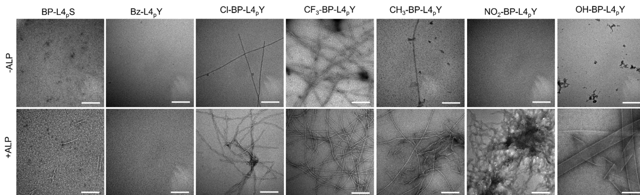
Fig. 5 TEM images of analogues of BP-L4pY (50 \mu\text{M} ) in PBS in the absence or presence of ALP (0.1 U mL -1 ) for 24 h. Scale bar: 200 nm.
