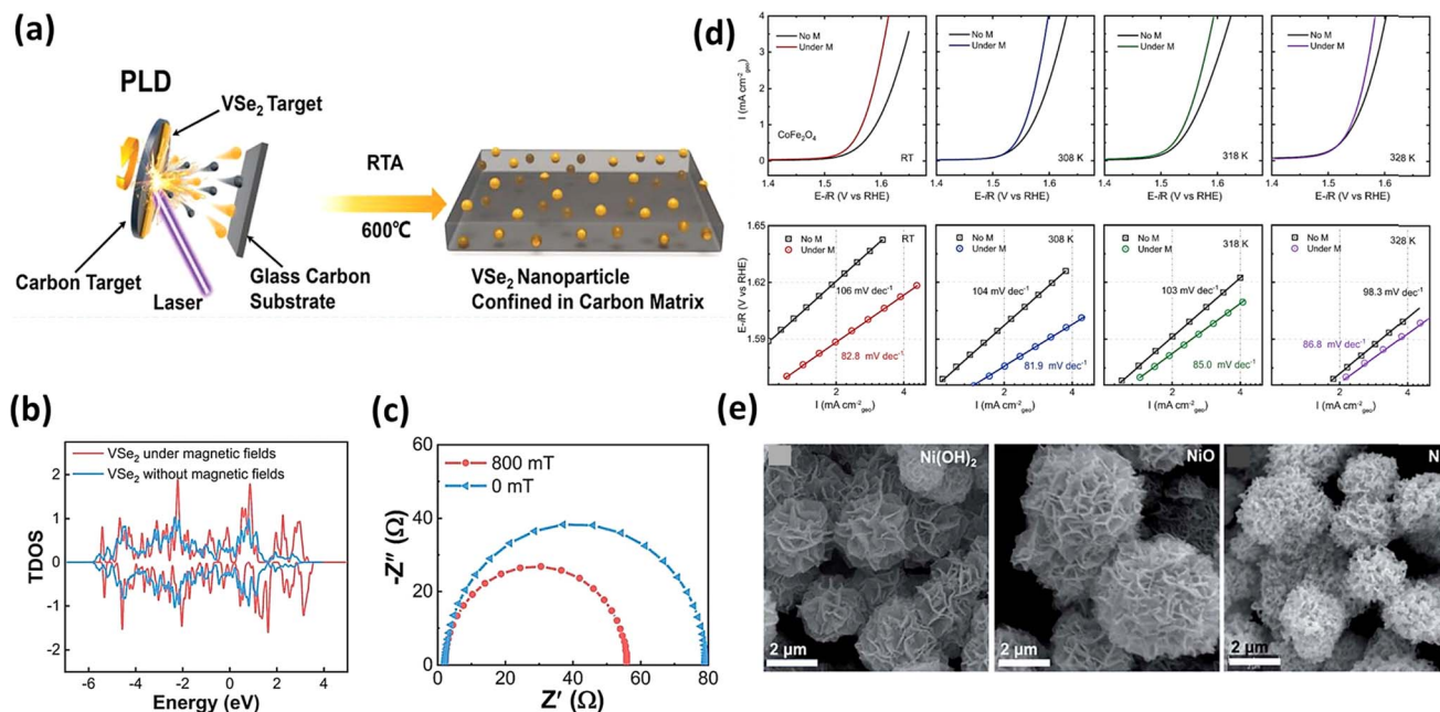
Fig. 19 (a) Schematic illustration of the synthesis of \text{VSe}_2 through pulsed laser deposition, (b) TDOS spectra of \text{VSe}_2 and (c) Nyquist plots of \text{VSe}_2 under a magnetic field of 0 and 800 mT (reprinted with permission, 199 copyright 2023, Wiley). (d) LSV curves and Tafel plots of \text{CoFe}_2\text{O}_4 at different temperatures (reprinted with permission, 122 copyrights 2021, Nature Communications ) and (e) SEM images of \text{Ni}(\text{OH})_2 , \text{NiO} and \text{Ni} (reprinted with permission, 200 copyright 2022, the Royal Society of Chemistry).
