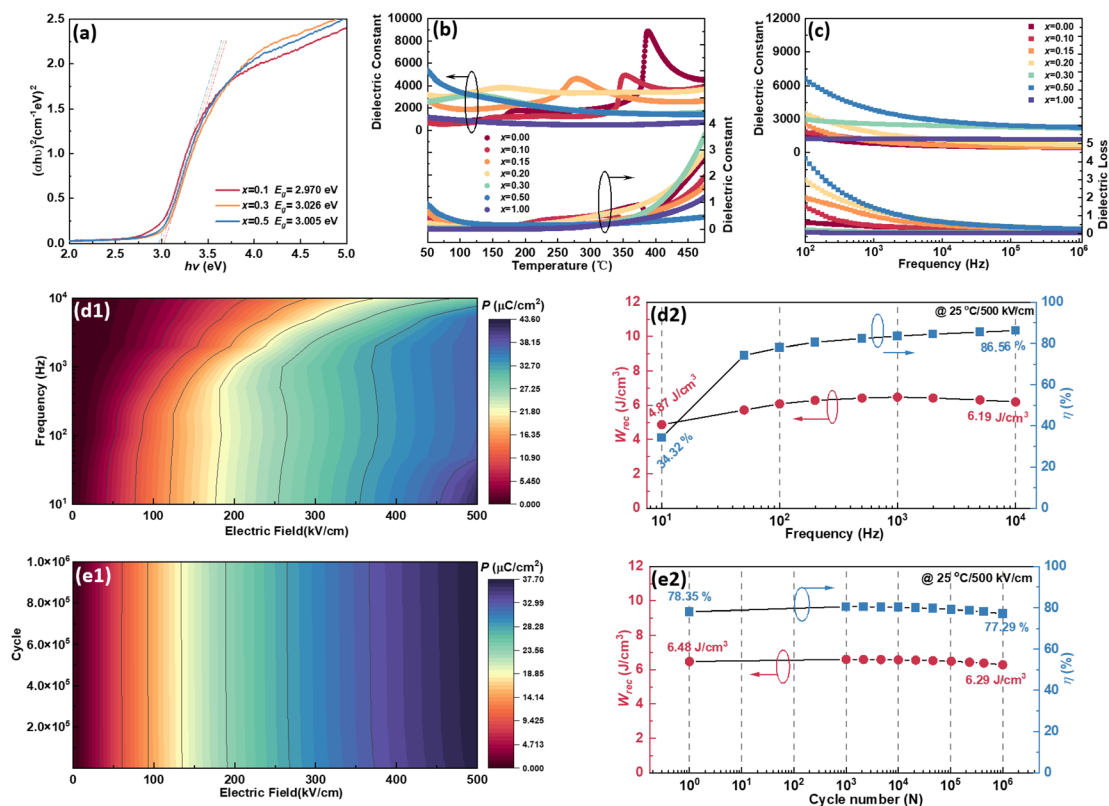
Fig. 6 (a) The fitting results of Fig. S6† according to eqn (15) to obtain the E_g of (1-x) KNN- x BCZT with x = 0.1, 0.3 , and 0.5 ; (b) the \varepsilon-T curves with \tan \delta-T curves of the (1-x) KNN- x BCZT ceramics from 50^\circ\text{C} to 475^\circ\text{C} at 1000\text{ Hz} ; (c) the \varepsilon-f curves with the \tan \delta-f curves of the (1-x) KNN- x BCZT ceramics from 10^2 to 10^6\text{ Hz} at room temperature; (d1) the mapping to show the variation between polarization and both the applied frequency and the electric field; (d2) the variation between both W_{\text{rec}} and \eta and frequency; (e1) the mapping to show the variation between polarization and both the cycling number and the electric field; (e2) the variation between both W_{\text{rec}} and \eta and the cycling number.
