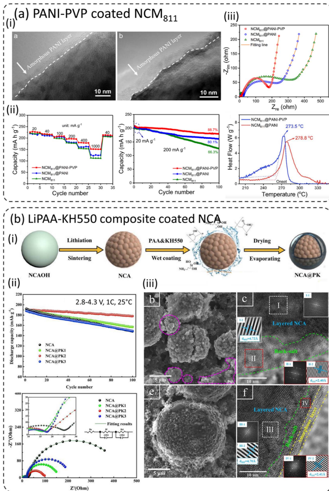
Fig. 7 (a) PANI–PVP coated \text{NCM}_{811} , (i) TEM image of the PANI–PVP coated \text{NCM}_{811} cathode material, (ii) rate capability and cycling performance comparison, and (iii) electrochemical impedance spectra (EIS) after the 100th cycle and DSC profiles of bare \text{NCM}_{811} and PANI–PVP– \text{NCM}_{811} , 35 reproduced from ref. 35 with permission from American Chemical Society, copyright 2019, (b) lithium polyacrylate (LiPAA) coated Ni-rich \text{LiNi}_{0.8}\text{Co}_{0.15}\text{Al}_{0.05}\text{O}_2 (NCA), (i) schematic illustration of the PAA coated NCA cathode, (ii) cycling and EIS spectra of bare and PAA–NCA cathodes after 100 cycles, and (iii) SEM and TEM images of bare and NCA@PK2 cathode particles after 100 cycles, 85 reproduced from ref. 85 with permission from Wiley, copyright 2020.
