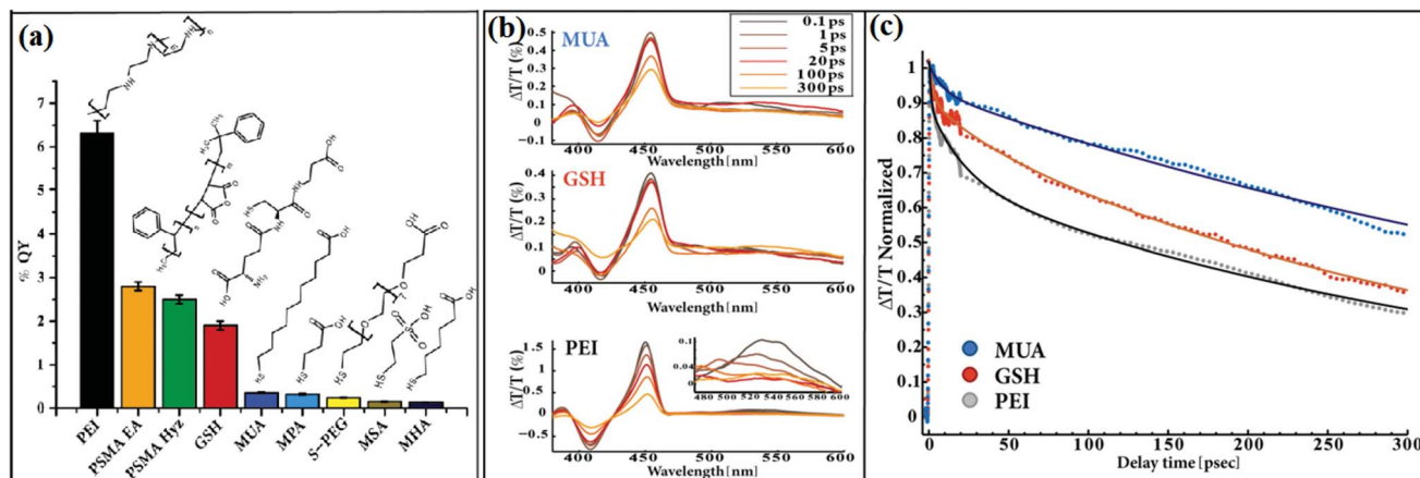
Fig. 20 (a) Apparent photocatalysis % QY values for a wide range of surface coatings, including thiolated alkyl ligands, GSH, and polymer coating. (b) Transient absorption spectra of CdS-Au NHPs for different surface coatings at 450 nm excitation. Expansion of the Au plasmon region for the PEI coating are presented in the inset (lower left frame). (c) Normalized transient absorption kinetics of the bleach recovery at 460 nm, corresponding to the first exciton transition of the CdS nanorod component, together with the exponential fits (continuous lines) for CdS-Au NHPs with different surface coatings. Reproduced with permission from ref. 99. Copyright 2015, Wiley.
