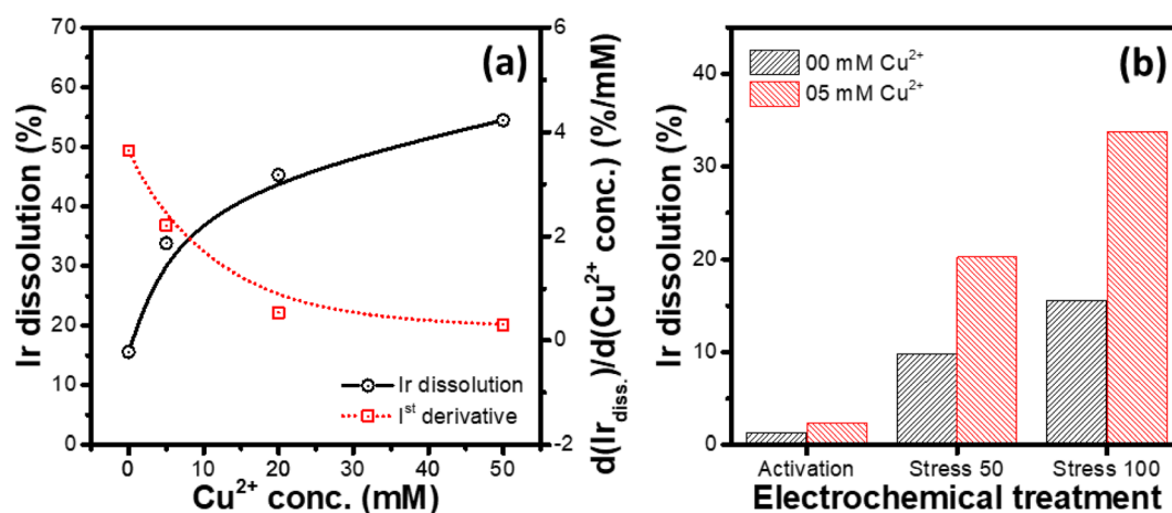
Fig. 5 (a) Variations of the Ir dissolution and its first derivative with the \text{Cu}^{2+} concentration. (b) Effect of different electrochemical treatments on the Ir dissolution (activation: 100 cycles, 1 V s -1 , 0–1.65 V; stress 50: activation + 50 stress cycles, 100 mV s -1 , 0–1.65 V; stress 100: activation + 100 stress cycles, 100 mV s -1 , 0–1.65 V) in 1 M HCl and 1 M HCl + 5 mM \text{CuCl}_2 electrolytes, respectively.
