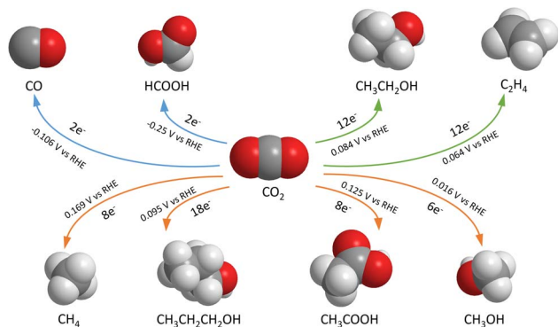
Fig. 1 Common electrochemical \text{CO}_2 reduction reaction products, number of electrons transferred and reaction standard potentials. 14
