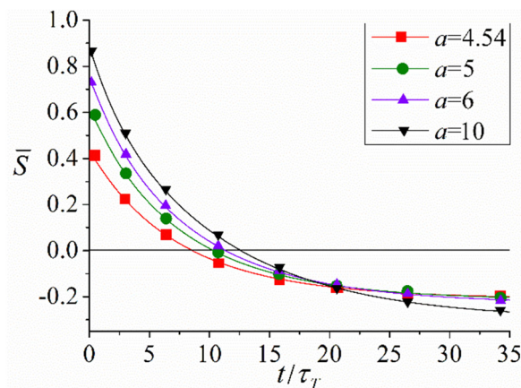
Fig. 13 Time dependences of the average order parameter \bar{S} at different strengths of LC interactions a and at fixed all other physical parameters: P_C/P_T = \bar{P}_C = 1 , D/P_T \equiv \bar{D} = 2 \times 10^{-2} , \chi = 20^\circ . The units of time: \tau_T = 1/P_T . Adapted from ref. 144. Copyright 2017 Royal Society of Chemistry.
