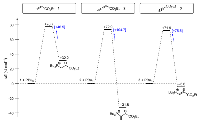
Fig. 18 Gibbs energy profiles for \text{PBU}_3 additions to Michael acceptors 1, 2 and 3 in dichloromethane solution. Experimentally determined Gibbs activation energies \Delta G_{\text{exp}}^\ddagger are combined with quantum-chemically calculated reaction energies \Delta G_{\text{add}} (data from Table 4). Reaction barriers for the retro-additions [\Delta G_{\text{retro}}^\ddagger] are given in square brackets.
