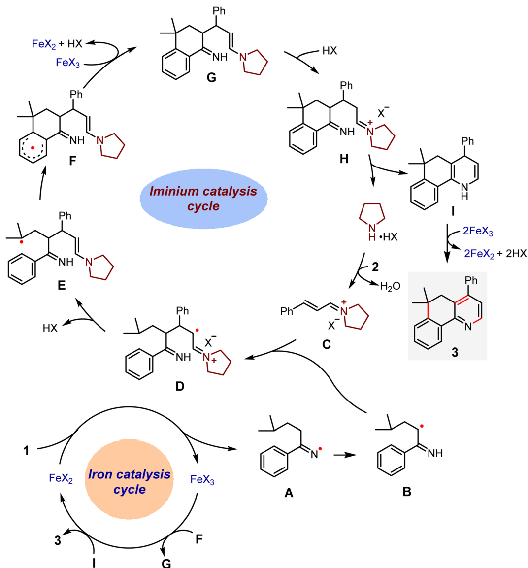
Scheme 7 Proposed mechanism for the relay annulation via synergistic iron and iminium catalysis ( X = \text{ClO}_4, \text{OBz}, or \text{acac} ).
