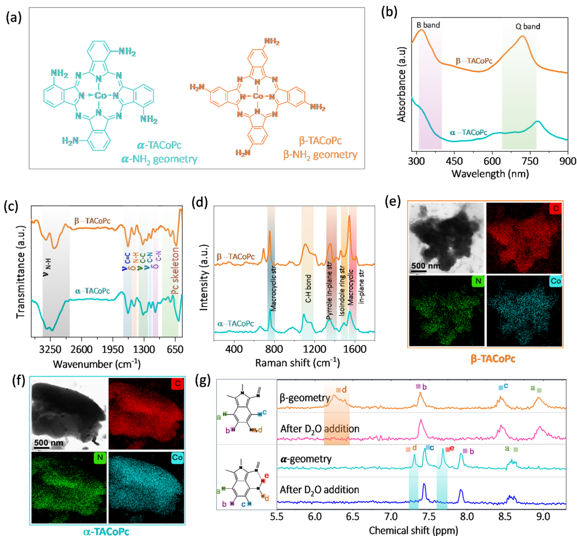
Fig. 1 Molecular structures of isomeric (a) \alpha -TACoPc and \beta -TACoPc molecules. (b) UV-vis spectra. (c) ATR-FTIR spectra, and (d) Raman spectra of isomeric \alpha -TACoPc and \beta -TACoPc molecules. HRTEM images and elemental mapping of (e) \beta -TACoPc and (f) \alpha -TACoPc molecules. (g) ^1\text{H} NMR spectra in \text{DMSO}-d_6 for the isomeric molecules before and after \text{D}_2\text{O} addition.
