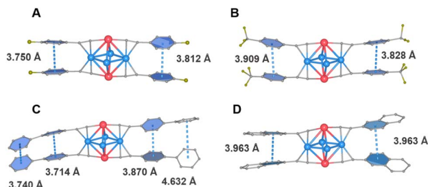
Fig. 6 The \pi\cdots\pi intramolecular interactions of (a) F-Cu 4 Pt 2 , (b) CF 3 -Cu 4 Pt 2 , (c) Biph-Cu 4 Pt 2 , and (d) Nap-Cu 4 Pt 2 .
