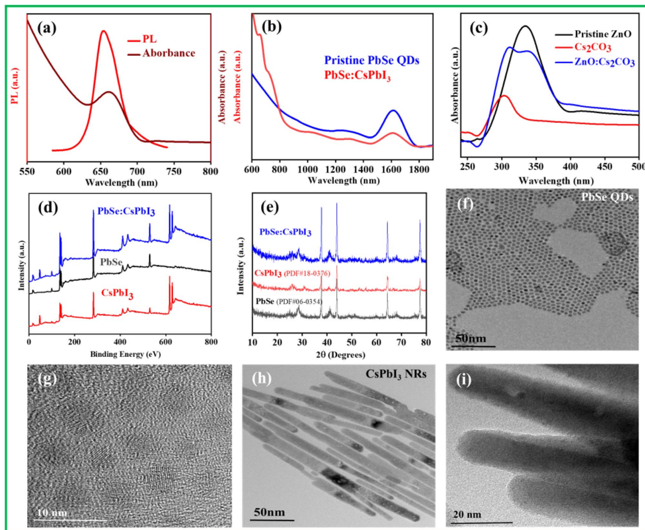
Fig. 1 Absorption and PL spectra of the as-synthesized CsPbI 3 NRs (a), absorption spectra of pristine PbSe QDs and their hybrid CsPbI 3 :PbSe nanocomposites (b), and pristine ZnO NPs and their hybrid Cs 2 CO 3 :ZnO nanocomposites (c). XPS spectra of pristine PbSe QDs, CsPbI 3 NRs and their CsPbI 3 :PbSe nanocomposite (d). XRD patterns of PbSe QDs, CsPbI 3 NCs, and their hybrid nanocomposites (e). TEM image of pristine PbSe QDs (f), and HRTEM image of PbSe QDs (g). TEM image of the pristine CsPbI 3 NRs (h), and the HRTEM image of CsPbI 3 NRs (i).
