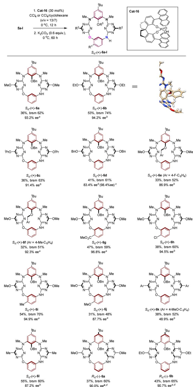
Scheme 3 Catalytic enantioselective synthesis of inherently chiral \text{N}_3,\text{O} -calix[2]arene[2]triazines 6a–l and the X-ray molecular structure of S_{1C} - 6b . a Reaction was performed in a mixture of \text{CCl}_4 and cyclohexane ( v/v = 13/7 ). b Reaction was carried out in pure \text{CCl}_4 . c The ee value was obtained after recrystallization. d Enantiomer of Cat-16 was used as the chiral catalyst.
