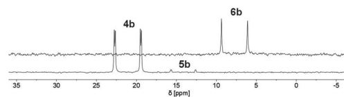
Fig. 7 31 P NMR spectra (CD 2 Cl 2 ) of 1,2-dihydrophosphinine oxide 4b (bottom) and its deprotonation product, phosphinine-1-olate 6b , after reaction with LDA (top).
