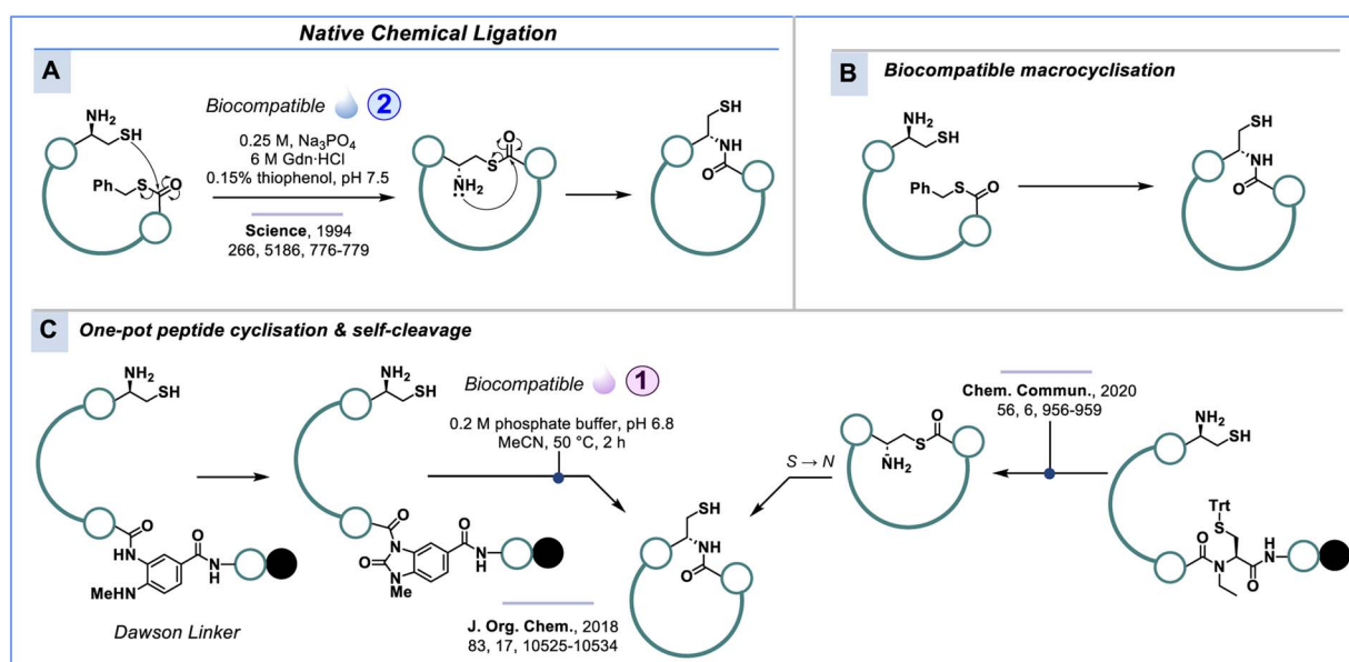
Scheme 7 Native chemical ligation (NCL). [A] Fundamental N -to- S acyl shift mechanism. [B] Biocompatible NCL with an N-terminal aminothioliol and C-terminal thioester. [C] Examples of NCL using safety catch linkers for direct on-resin C-terminal modification.
