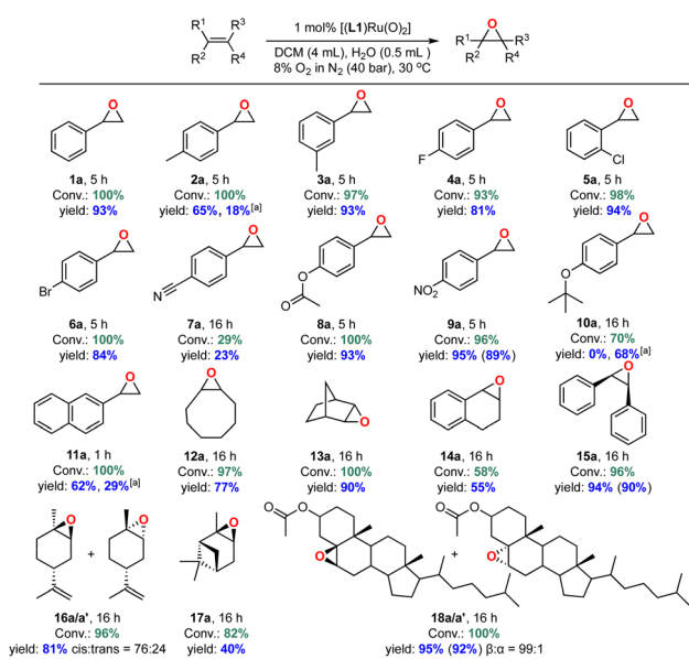
Fig. 13 Substrate scope of [(\mathbf{L1})\text{Ru}^{\text{VI}}(\text{O})_2(\text{H}_2\text{O})_2] catalysed aerobic alkene epoxidation. Conversions and yields determined by quantitative 1 H NMR spectroscopy against mesitylene as internal standard; isolated yields provided in parentheses. [a] Yield of corresponding aldehyde from epoxide isomerisation.
