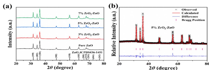
Fig. 3 (a) XRD patterns of the pure ZnO and x% \text{ZrO}_2\text{-ZnO} ( x = 3, 5, 7 ) samples. (b) Rietveld plots with 5% \text{ZrO}_2\text{-ZnO} .
