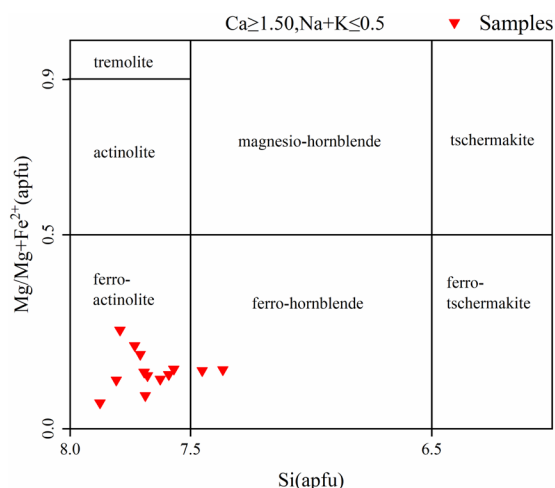
Fig. 8 Diagram of amphibole classification (adapted from Leake et al. , 1997 (ref. 36)) (apfu = atoms per formula unit).
