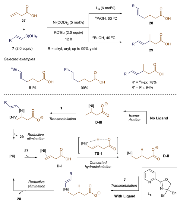
Scheme 7 Regiodivergent hydroalkenylation.
