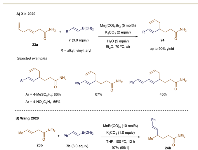
Scheme 5 Mn(I)-catalyzed hydroalkenylation of unbiased internal alkenes.
