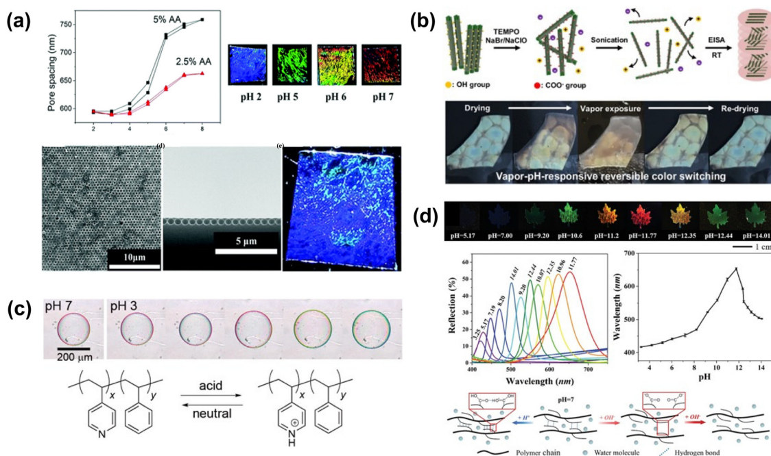
Fig. 22 (a) pH-dependent color change of the 2D inverse opal hydrogel via pH modulated pore spacing. [Reproduced from ref. 199, with permission from Royal Society of Chemistry, Copyright 2014]. (b) Schematic of the fabrication of oxidized CNC (OxCNC) films by evaporation-induced self-assembly. PEG/OxCNC composite film undergoes reversible color change upon vapor exposure. [Reproduced from ref. 200, with permission from Elsevier Publishing Group, Copyright 2019]. (c) Schematic illustration showing the mechanism of pH responsiveness for the films assembled by the copolymer nanoparticles. [Reproduced from ref. 202, with permission from American Chemical Society, Copyright 2016]. (d) Color and reflection spectra of the leaf pattern in response to solution with different pH value. [Reproduced from ref. 201, with permission from Wiley-VCH Verlag GmbH & Co. KGaA, Weinheim, Copyright 2019].
