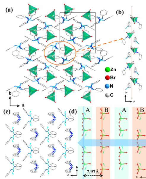
Fig. 1 (a) The structure of 1 along the c -axis; (b) the inorganic and organic parts rotating along the c axis with 2_1 helical arrangement; (c) the organic layers parallel with the ac plane; (d) the inorganic layers in the bc plane and their distance. Hydrogen atoms are omitted for clarity.
