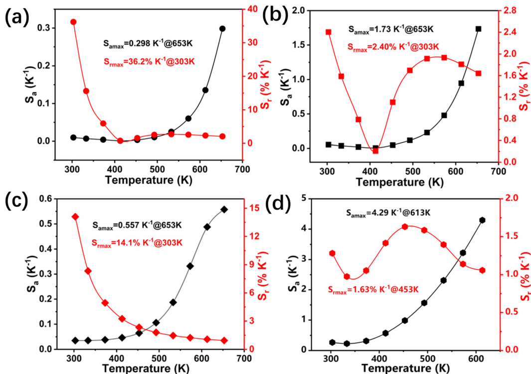
Fig. 5 Calculated S_a and S_r values of the NaLa 0.89 Ti 2 O 6 :0.10Yb 3+ ,0.01Tm 3+ phosphor based on the FIR of I_{696}/I_{474} (a), I_{800}/I_{474} (b), I_{696}/I_{650} (c), and I_{800}/I_{650} (d).
