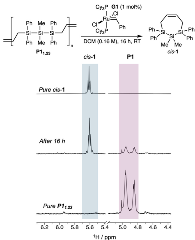
Fig. 3 Cropped ^1\text{H} NMR spectra of pure cis -1 (top), after 16 hours of depolymerization (middle), and pure P1 (bottom) showing 55% depolymerization to cis -1.
