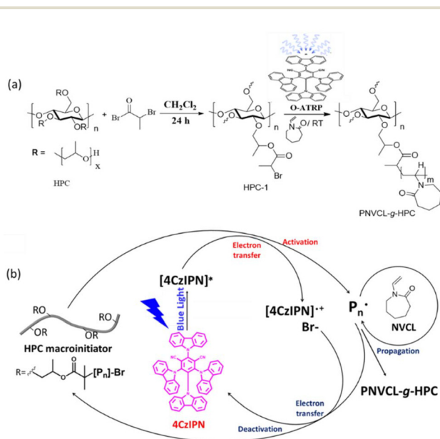
Scheme 1 (a) Preparation of PNVCL- g -HPCs polymer. (b) The O-ATRP mechanism.
