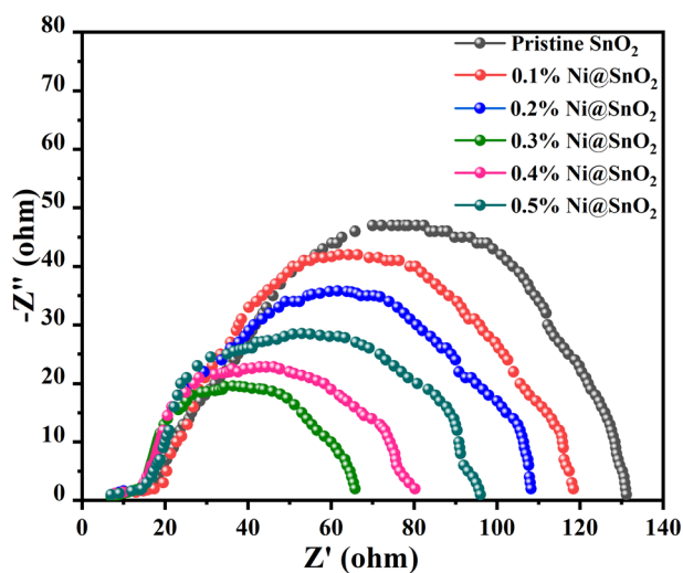
Fig. 12 Nyquist plot for SnO 2 and 0.1 to 0.5% Ni@SnO 2 nanostructures.
