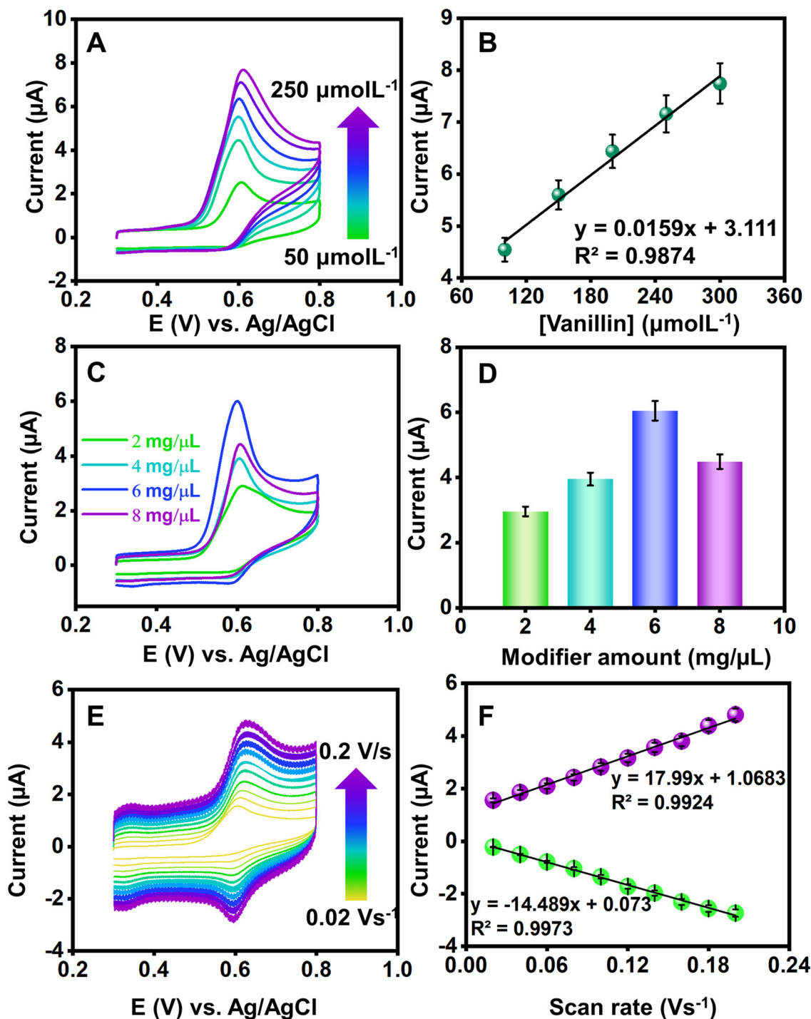
Fig. 5 (A) CV profile of \text{NdNbO}_4/\text{f-CNF}/\text{GCE} for increasing concentrations of VAN ( 50\text{--}250\ \mu\text{mol L}^{-1} ); (B) calibration plot of VAN concentration versus anodic peak current; (C) CV profile obtained for different loading amounts of the \text{NdNbO}_4/\text{f-CNF} nanocomposite over the GCE; (D) plot of loading amount versus anodic peak currents; (E) CV profile of 100\ \mu\text{mol L}^{-1} VAN for varying scan rates from 0.02 to 0.2\ \text{V s}^{-1} ; and (F) calibration plot of increasing scan rates versus redox peak currents.
