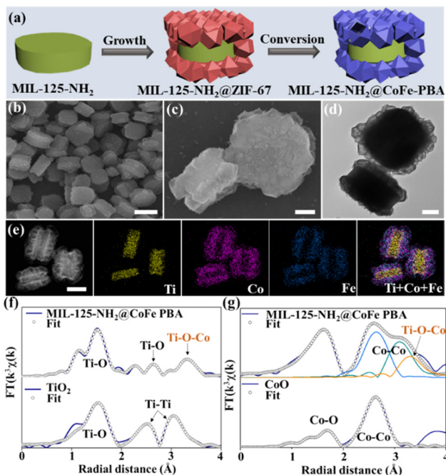
Fig. 10 (a) Illustration of the synthesis process of MIL-125-NH 2 @CoFe PBA. (b and c) SEM, (d) TEM, (e) HAADF-STEM and the corresponding elemental mapping images. Scale bars are: (b), 1 \mu\text{m} ; (e), 500 nm; and (c and d), 200 nm. (f) Ti coordination environments of MIL-125-NH 2 @CoFe PBA and TiO 2 and (g) Co coordination environments of MIL-125-NH 2 @CoFe PBA and CoO. Reprinted with permission from ref. 44. Copyright 2023 Wiley-VCH.
