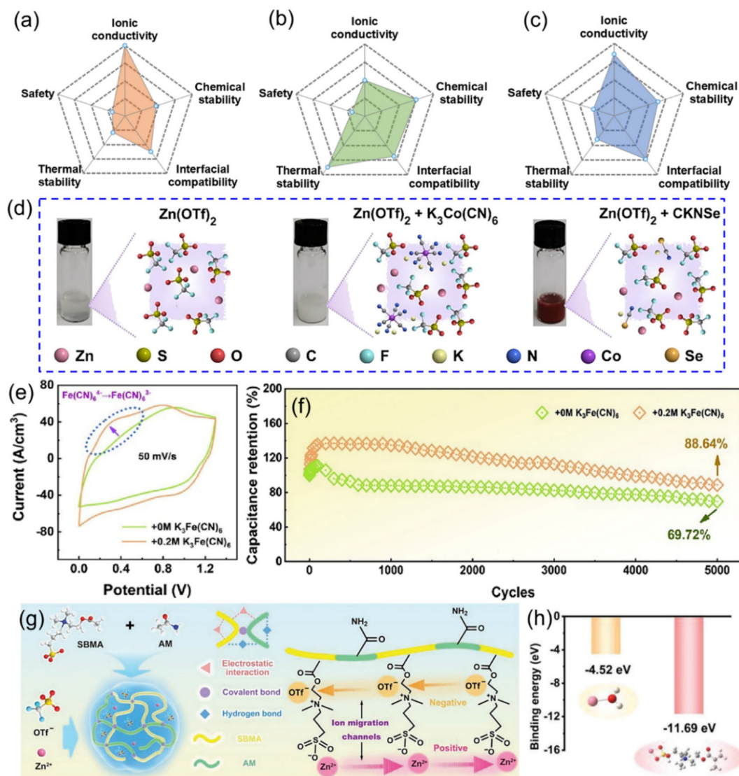
Fig. 8 Radar maps showing the comparison of (a) aqueous electrolyte, (b) organic electrolyte, and (c) gel electrolyte, respectively. (d) Photos and molecular structures of the pure \text{Zn(OTf)}_2 electrolyte and hybrid electrolytes containing \text{K}_3\text{Co(CN)}_6 or \text{CKNSe} additives. Reproduced with permission from ref. 87. Copyright 2023, The Royal Society of Chemistry. (e) CV curves tested in \text{KFCN}_0 and \text{KFCN}_{0.2} electrolytes. (f) Cycling stability of \text{Ti}_3\text{C}_2\text{T}_x -DMAC MXene-based ZIHMSCs separately tested in \text{KFCN}_0 and \text{KFCN}_{0.2} electrolytes. Reproduced with permission from ref. 113. Copyright 2023, American Chemical Society. (g) Schematic diagram of fabrication, cross-linked structure, and ion migration channels of PASHE consisting of \text{P(AM-co-SBMA)} polymeric skeleton and \text{Zn(OTf)}_2 electrolyte. (h) Binding energies of \text{Zn}^{2+} - \text{H}_2\text{O} and \text{Zn}^{2+} -PASHE based on simulation. Reproduced with permission from ref. 114. Copyright 2022, WILEY-VCH.
