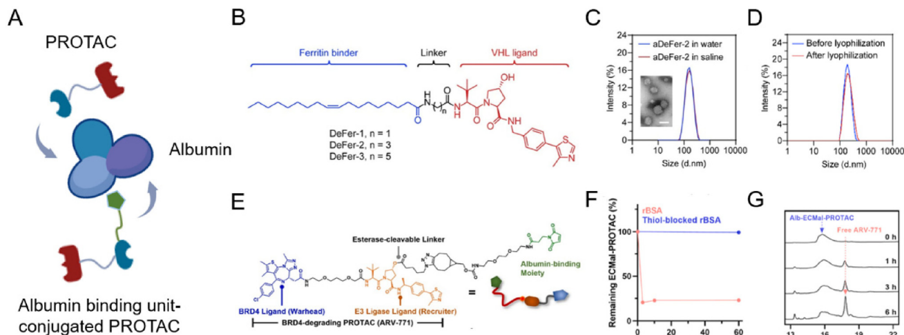
Fig. 7 (A) Schematic depiction of the preparation of an albumin-encapsulated PROTAC delivery system. (B) Chemical structures of oleic acid-based VHL-recruiting PROTACs. (C) Size distribution of aDeFer-2 in water and saline and the morphology observed by TEM. Scale bar, 100 nm. (D) Size distribution of aDeFer-2 before and after lyophilization. Reproduced from ref. 78 with permission. Copyright 2023, American Chemical Society. (E) Chemical structures of albumin-binding moiety-modified BRD4-degrading PROTACs. (F) The HPLC peak of Alb-ECMal after incubation with BSA and thiol-blocked BSA. (G) The HPLC peak of Alb-ECMal PROTAC with an esterase solution ( 30 \text{ U mL}^{-1} ). Reproduced from ref. 81 with permission. Copyright 2023, Elsevier.
