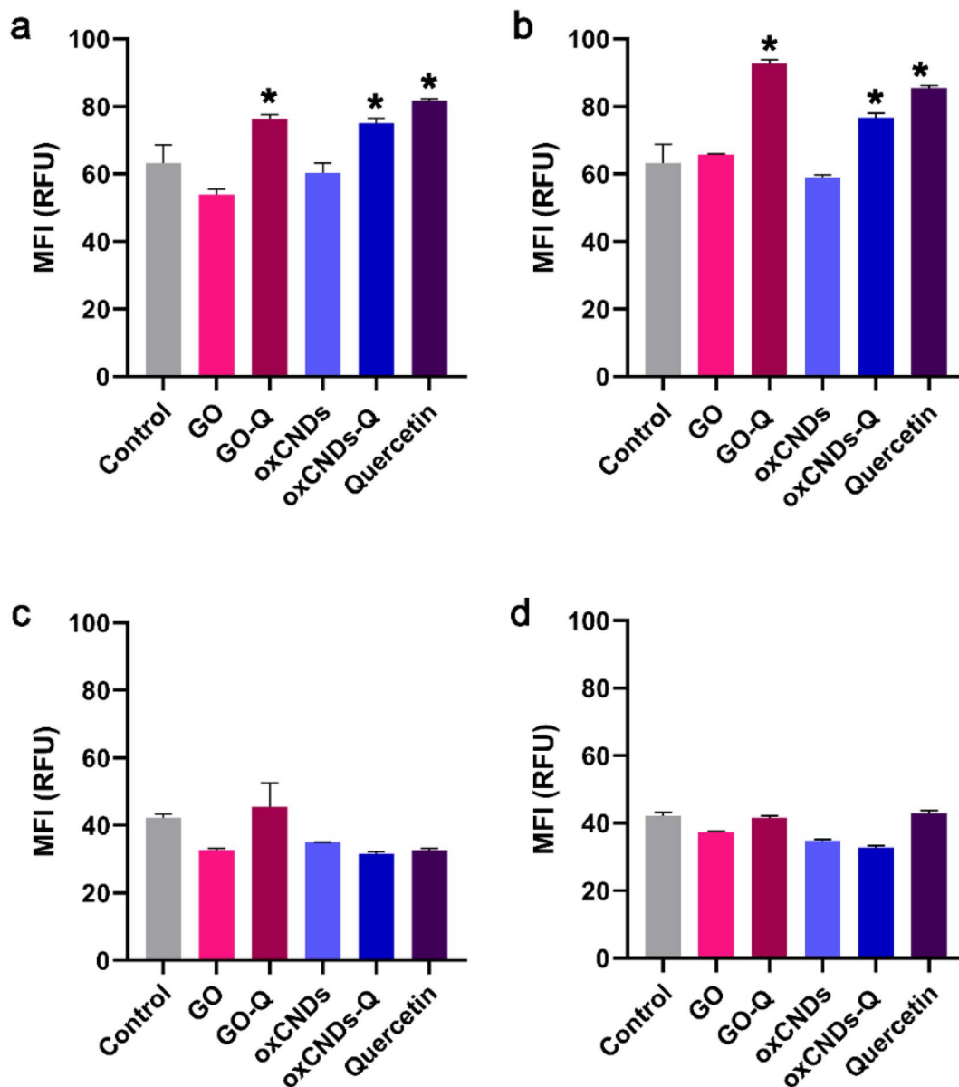
Fig. 12 ROS production in NIH/3T3 (a and b) and U87 cells (c and d) after treatment with either 1\text{ }\mu\text{g mL}^{-1} (a and c) or 10\text{ }\mu\text{g mL}^{-1} (b and d) of GO, GO-Q, oxCNDs, oxCNDs_Q or quercetin alone, for 24 h. MFI, mean fluorescence intensity. RFU, relative fluorescence units. *, statistically significant difference from the control, p < 0.05 .
