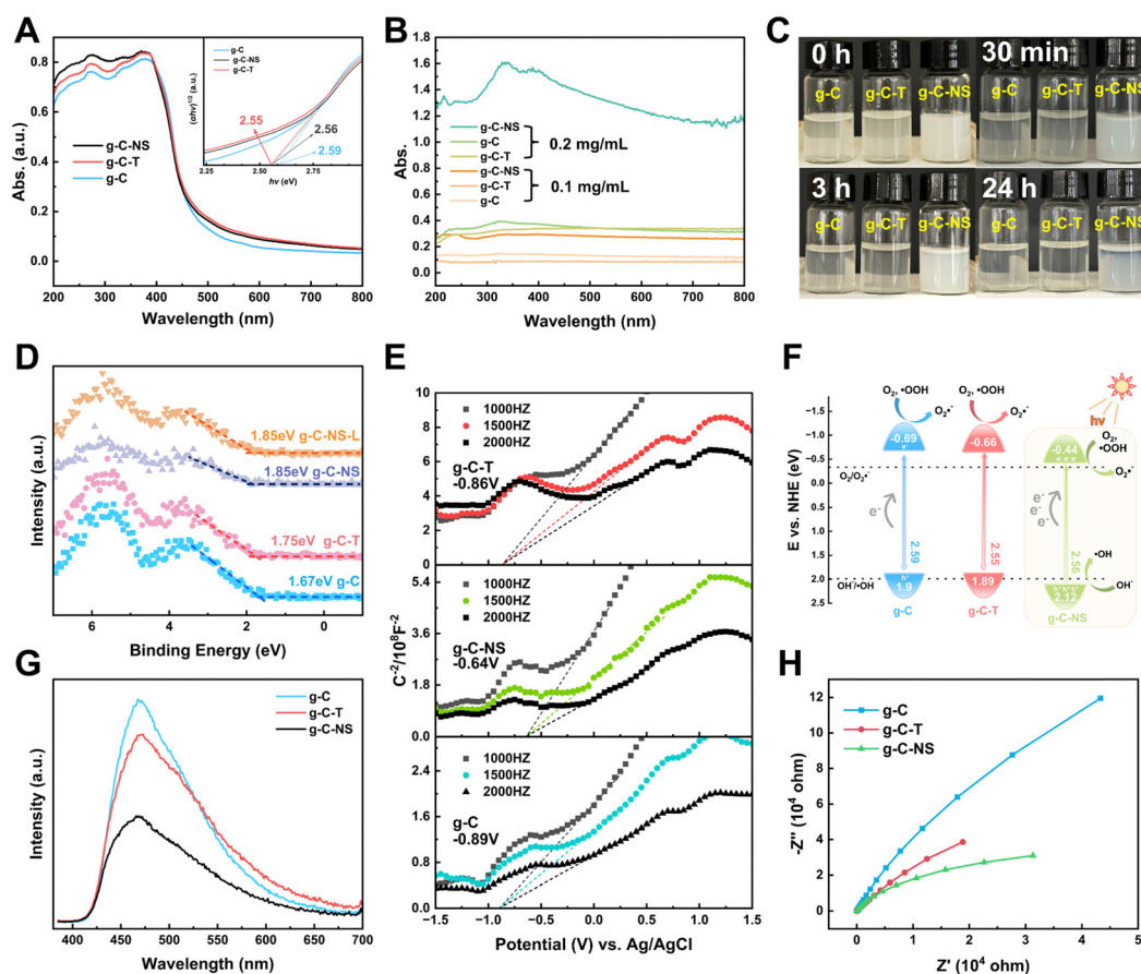
Fig. 4 (A) UV-vis DRS spectra (inset: plots of (\alpha h\nu)^2 versus h\nu ). (B) Absorption spectra of photocatalyst suspensions. (C) Photocatalyst suspensions. (D) XPS-VB spectra. (E) Mott–Schottky plots. (F) Band energy levels. (G) PL spectra. (H) Electrochemical impedance spectra (EIS).
