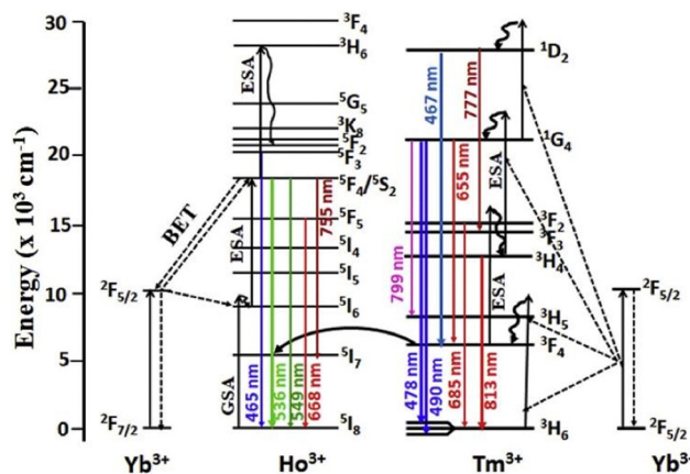
Fig. 7 Energy level diagrams of Ho 3+ -Yb 3+ -Tm 3+ ions and the possible UC and ET processes under 976 nm excitation. Reprinted with permission from Elsevier. 60
