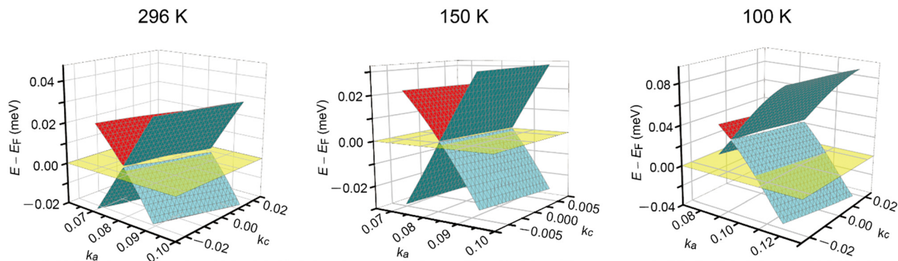
Fig. 2 Band structures near the Fermi level E_F in \alpha - \text{ET}_2\text{I}_3 at 1 bar and 296, 150, and 100 K in the k_a k_c space. At each T , the Fermi level is shown by the half-transparent yellow plane. The green (front)/red (back) and blue (front)/green (back) curved surfaces respectively show a part of the top and the second HOMO bands. The corresponding figure (the band structures in the k_a k_b space at 296, 150, and 100 K) is shown in Fig. S1 in the ESI ^\dagger which also shows linearly dispersive parts in the band structure.
