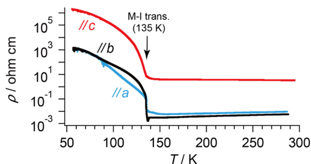
Fig. 4 T -dependent electrical resistivities of \alpha - \text{ET}_2\text{I}_3 along each crystallographic axis. The values are identical at T \approx 60 –90 K along the a - and b -axes.
