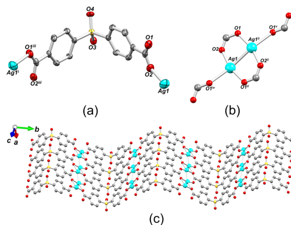
Fig. 2 Structural representations of 1 . (a) Connectivity of μ 6 -sdba 2− ligand. (b) Coordination environment around Ag1 centers (some atoms are omitted for clarity). Symmetry code: i (−1 − x , \frac{1}{2} + y , 1 − z ); ii (−1 − x , 1 − y , 1 − z ); iii ( x , \frac{1}{2} − y , z ); iv ( x , y , 1 + z ); v (−1 − x , 1 − y , − z ). (c) 2D metal–organic layer along the bc plane. Ag (cyan), O (red), S (yellow), C (gray).
