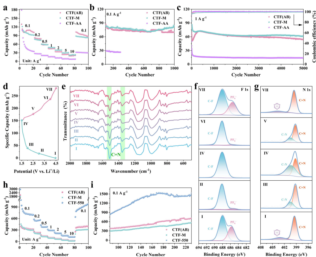
Fig. 2 (a) Rate performance of CTF, CTF-M, and CTF-AA as the cathode at various current densities. (b) Cycling performance of CTF, CTF-M, and CTF-AA as the cathode at 0.1 A g -1 . (c) Long-term cycling stability of CTF, CTF-M, and CTF-AA as the cathode at 1 A g -1 . Ex situ characterization of the CTF electrode as the cathode at different discharge and charge states: (d) charge/discharge curves; (e) FT-IR spectra of CTF; (f) F 1s XPS spectra of CTF; (g) N 1s XPS spectra of CTF. (h) Rate performance of CTF, CTF-M, and CTF-550 as the anode in the voltage range of 0.005–3 V at various current densities. (i) Cycling performance of CTF, CTF-M, and CTF-550 as the anode at 0.1 A g -1 .
