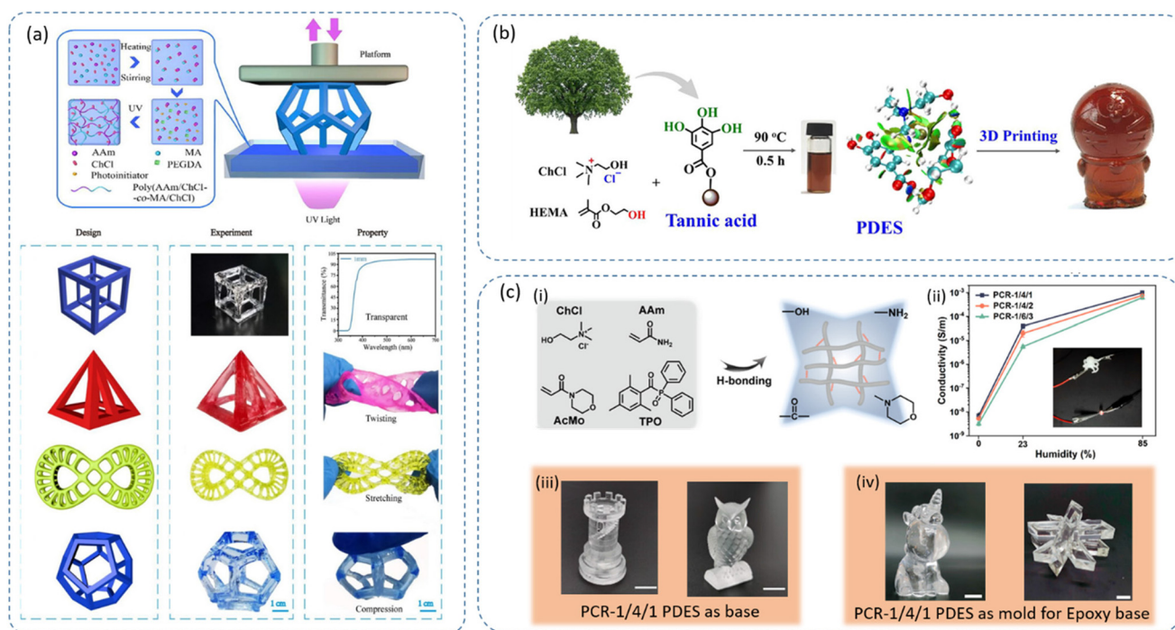
Fig. 9 Photocurable resins generated by PDESs for 3D printing applications. (a) Schematic illustration of SLA printing of a PDES (acrylamide:ChCl:maleic acid) and 3D printed models for conductive elastomeric sensors. 156 Copyright 2021, Elsevier. (b) LCD 3D printing of a bio-based PDES (ChCl:HEMA). 163 Copyright 2023, American Chemical Society. (c) (i) Composition and hydrogen bonding in a PDES (ChCl:acrylamide:4-acryloylmorpholine). (ii) Conductivity variations with respect to humidity from 0–85%. (iii) Structures generated by the LCD 3D printing of PCR 1/4/1 (ChCl:acrylamide:4-acryloylmorpholine, 1:4:1). (iv) Epoxy structures generated by 3D printed PCR 1/4/1 sacrificial molds. 161 Copyright 2023, American Chemical Society.
