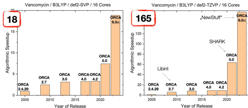
Fig. 1 Algorithmic speedup over time relative to the early ORCA versions of 2005. The respective versions were all compiled with the same compiler, linked against the same libraries and run on the same computer. The test molecule was Vancomycin with 176 atoms. Left: def2-SVP basis set, right: def2-TZVP basis set.
