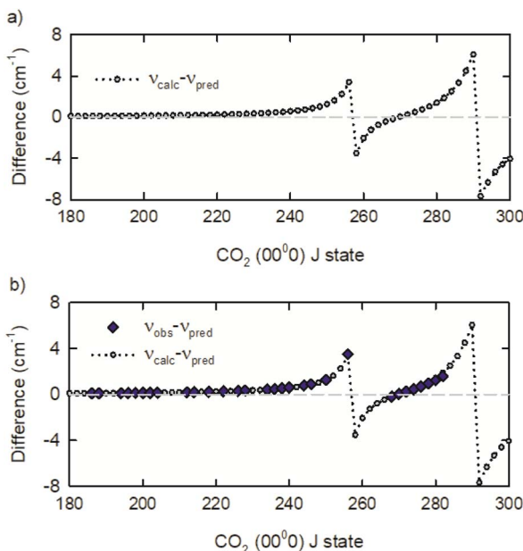
Fig. 4 (a) A comparison of calculated ( \nu_{\text{calc}} ) and predicted ( \nu_{\text{pred}} ) transition frequencies for CO 2 R-branch transitions. (b) A comparison of observed transition frequencies \nu_{\text{obs}} with the calculated and predicted values.
