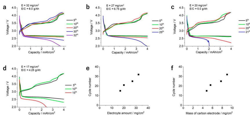
Fig. 3 Discharge/charge profile of LOB cells with different electrolyte amounts using the carbon electrodes with different thicknesses. (a) Electrolyte amount of 32 \text{ mg cm}^{-2} , carbon electrode thickness of 450 \mu\text{m} , (b) electrolyte amount of 27 \text{ mg cm}^{-2} , carbon electrode thickness of 380 \mu\text{m} , (c) electrolyte amount of 20 \text{ mg cm}^{-2} , carbon electrode thickness of 280 \mu\text{m} , and (d) electrolyte amount of 17 \text{ mg cm}^{-2} , carbon electrode thickness of 220 \mu\text{m} . (e) Relationship between the electrolyte amount and cycle number of the LOB cells. (f) Relationship between the mass of the carbon electrode and cycle number of the LOB cells.
