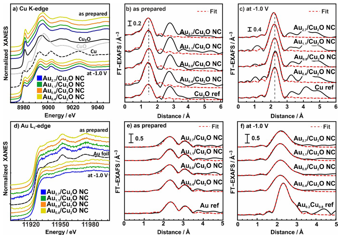
Fig. 4 Normalized XANES spectra from (a) the Cu K-edge and (d) Au-L 3 edge of bimetallic AuCu NCs with different Au:Cu ratios measured as-prepared and under CO 2 RR at -1 V_{\text{RHE}} , plotted together with bulk Cu, Cu 2 O and CuO references. FT-EXAFS data from the Cu K-edge (b) and (c) and Au-L 3 edge (e) and (f) are also shown together with the corresponding fits for the as-prepared samples (b) and (e) and those during 4 h of CO 2 RR (c) and (f). Reference EXAFS spectra of an Au foil and a Cu 0.2 Au 0.8 reference alloy are shown for comparison. Cu 0.2 Au 0.8 reference was redrawn from ref. 46.
