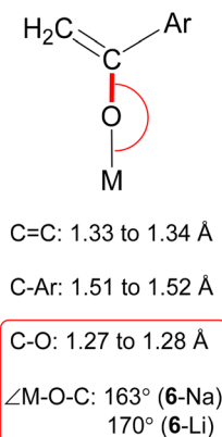
Scheme 4 Comparing the bond lengths in the enolate units of the hexamers and the monomers. The most pronounced structural changes are observed in the C-O bond length and the M-O-C bond angle (highlighted in red).
