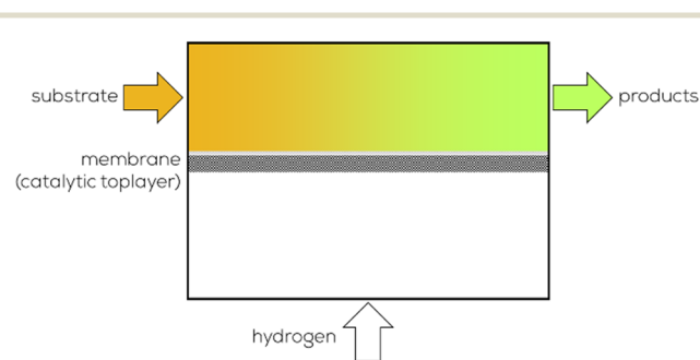
Fig. 43 Crossflow configuration for membrane reactors as used by Rezac. 205
