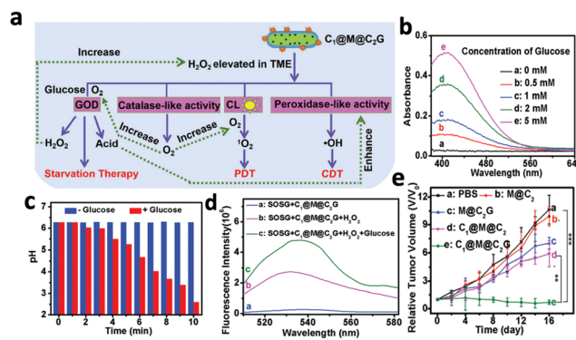
Fig. 6 (a) Schematic illustrations of the enhanced PDT by \text{C}_1\text{@M@C}_2\text{G} through enhanced generation of \text{H}_2\text{O}_2 combined with other therapies. (b) Absorption spectra of \text{C}_1\text{@M@C}_2\text{G} particles and glucose, where higher absorbance refers to higher \text{H}_2\text{O}_2 content. (c) pH measurement of the \text{C}_1\text{@M@C}_2\text{G} particle following addition of glucose ( 1 \text{ mg mL}^{-1} ) over time. (d) Fluorescence spectra of SOSG ( ^1\text{O}_2 indicator) added to \text{C}_1\text{@M@C}_2\text{G} after mixing with \text{H}_2\text{O}_2 and glucose, where higher fluorescence indicates higher ^1\text{O}_2 production. (e) In vivo tumour growth curves of mouse groups with different treatments. Reproduced with permission from ref. 54. Copyright 2021, Royal Society of Chemistry.
