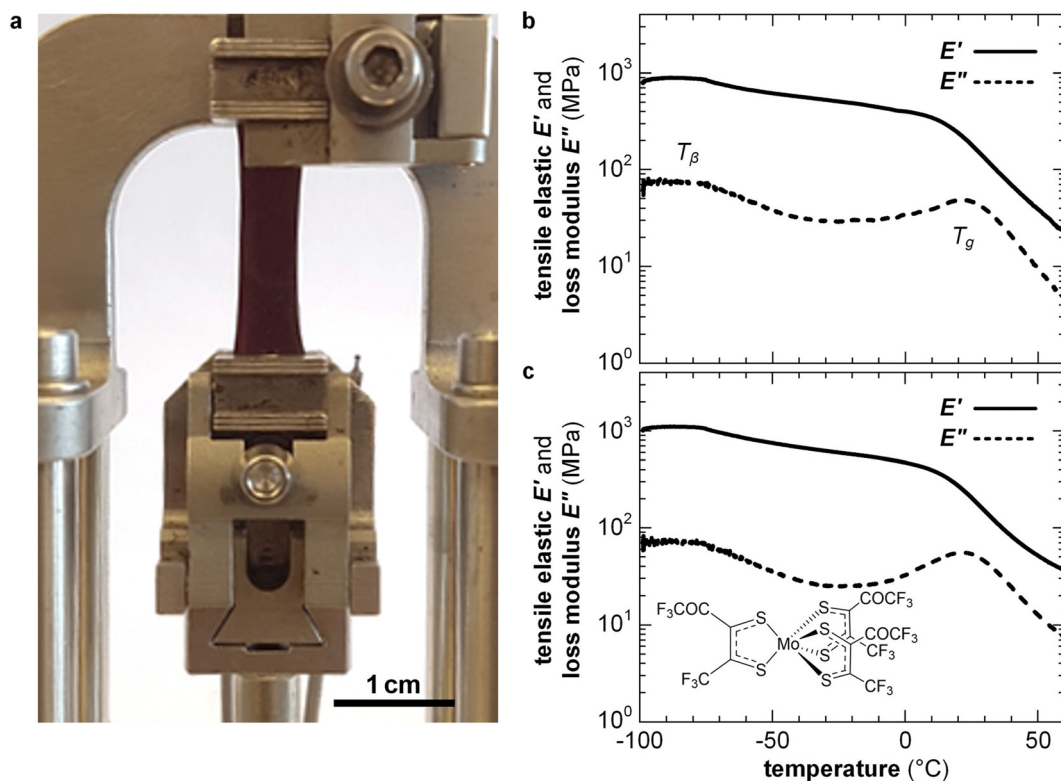
Fig. 14 (a) A tensile-drawn regio-regular P3HT film clamped in a dynamic mechanical analyzer, and DMA thermograms of isotropic P3HT films (b) prior to doping and (c) after sequential doping with \text{Mo}(\text{tfd-COCF}_3)_3 . Figure adapted with permission from ref. 38; Copyright 2019, American Chemical Society.
