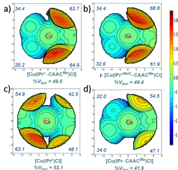
Fig. 5 Steric maps of (a) [\text{Cu}(\text{IPr}^*-\text{CAAC}^{\text{Me}})\text{Cl}] , (b) [\text{Cu}(\text{IPr}^{*\text{MeO}}-\text{CAAC}^{\text{Me}})\text{Cl}] , (c) [\text{Cu}(\text{IPr}^*)\text{Cl}] , and (d) [\text{Cu}(\text{IPr}-\text{CAAC}^{\text{Me}})\text{Cl}] showing \%V_{\text{Bur}} per quadrant. Adapted with permission. 230 Copyright © 2022, Royal Chemical Society.
