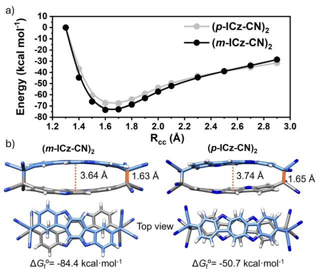
Fig. 2 (a) Potential energy curve (PES) scan of ( p -ICz-CN) 2 and ( m -ICz-CN) 2 in gas phase computed at the (U)M06-2X/6-31G** level. Here R_{\text{CC}} is the length of the C–C \sigma -bonds formed between two ICz units. (b) Lateral and top view of the DFT-calculated global minimum structure for ( m -ICz-CN) 2 (left) and ( p -ICz-CN) 2 (right) displaying the distances of the closest C–C \sigma -bonds and \pi - \pi interactions between the co-facially oriented monomers. The N -substituted alkyl groups have been omitted for clarity. Free energies of formation ( \Delta G_f^\circ ) of the ( m -ICz-CN) 2 and ( p -ICz-CN) 2 are also shown.
