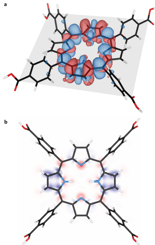
Fig. 4 Differential electron density of TCPP. (a) Difference in electron density (increased electron density in red, decreased density in blue) between ground state \text{S}_0 and excited triple state \text{T}_1 . The porphyrin plane is indicated in grey. (b) Differential electron density in the porphyrin plane. Red indicates an increase and blue a decrease in electron density.
